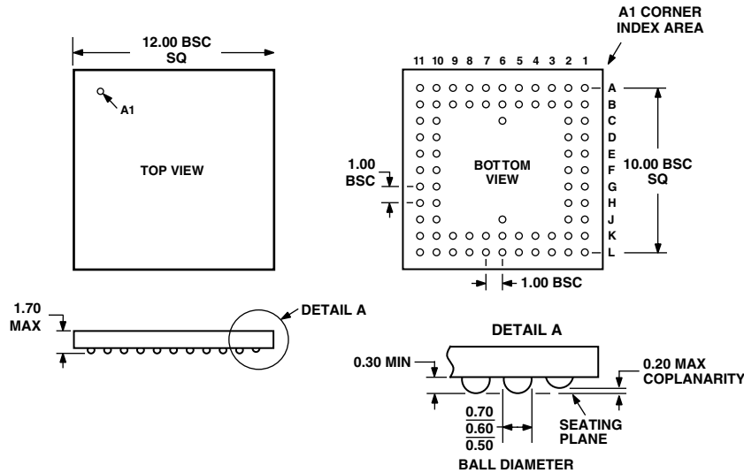
COMPLIANT TO JEDEC STANDARDS MO-192ABD-1
