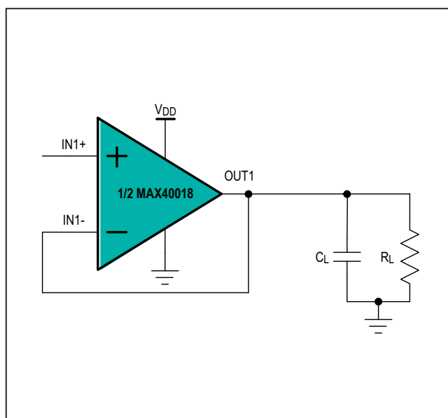
Figure 2. RL Improving Capacitive Load Drive Capability of Op Amp
