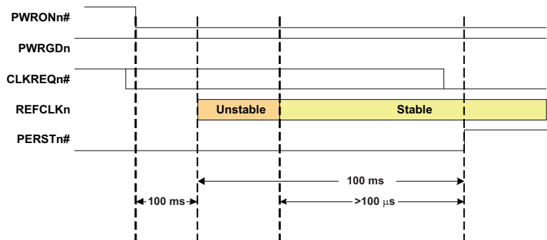
Figure 5-3. PCI Hot Plug Power-Up Cycle With No \text{PWGRDn} Feedback
