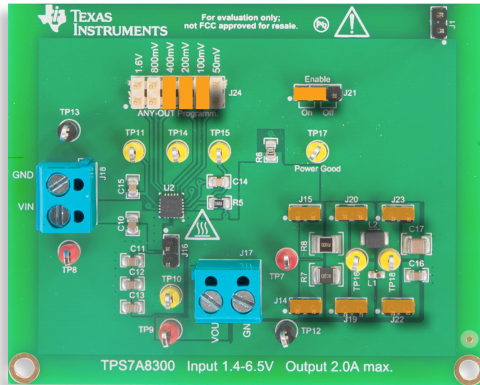
Figure 9. TPS7A8300 LDO board: jumpers set-up for Test#2
