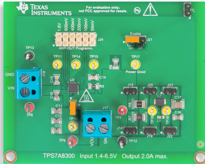
Figure 7. TPS7A8300 LDO board: jumpers set-up for Test#2
