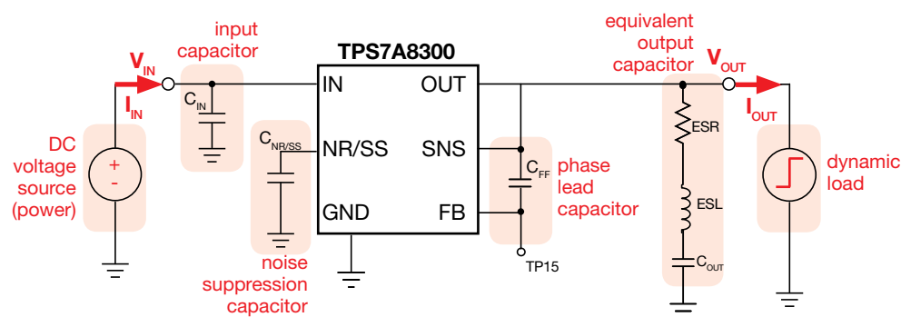
Figure 1. Simplified schematic of the TPS7A8300 LDO regulator
