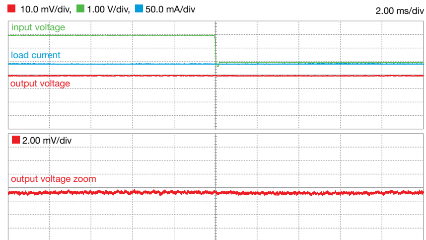
Figure 11. TPS7A4901 LDO line transient for V_{out}=5V , I_{OUT}=50mA , C_{FF}=12nF and V_{IN} falling from 8V to 6V
