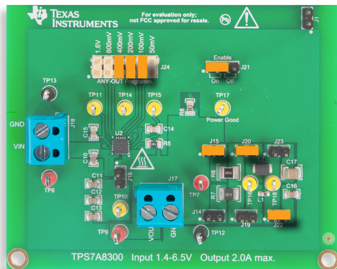
Figure 8. TPS7A8300 LDO board: jumpers set-up for Test#1
