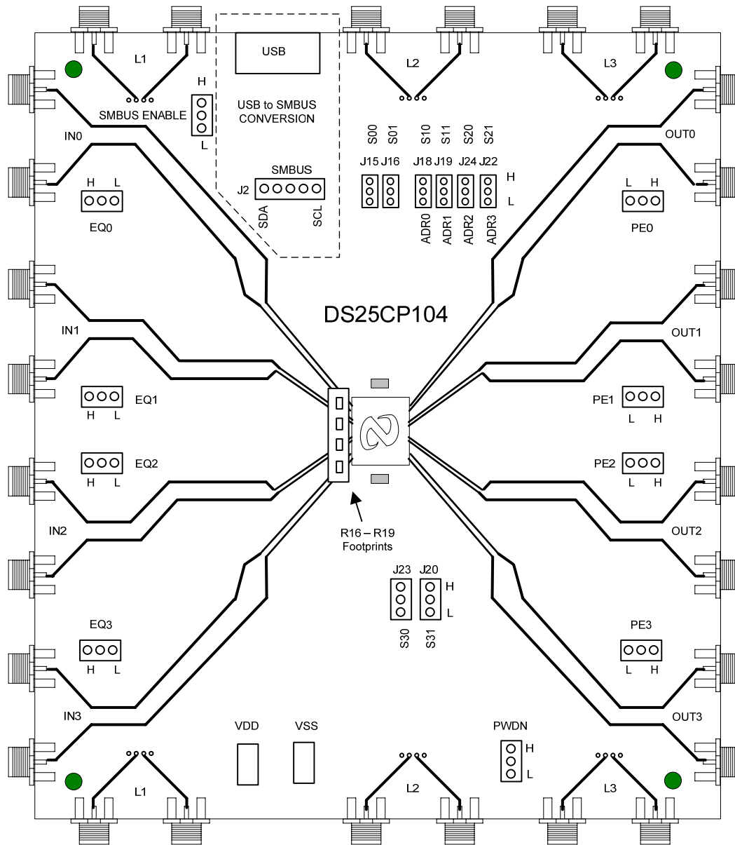
Figure 2. Top Layer DS25CP104EVK
