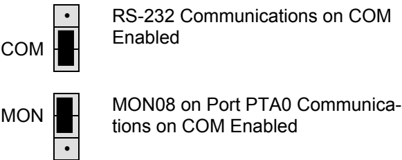
Figure 4: COM_MODE Jumper
