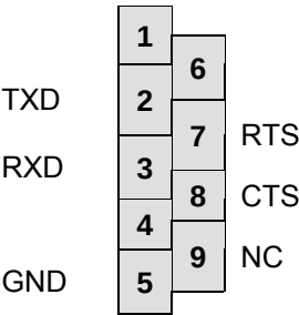
Figure 3: COM Connector
