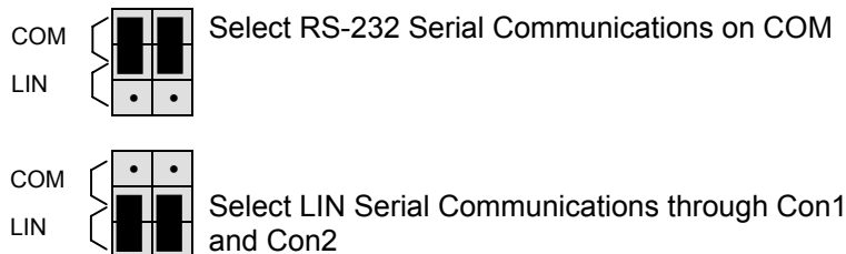
Figure 5: COM_SEL Jumper
