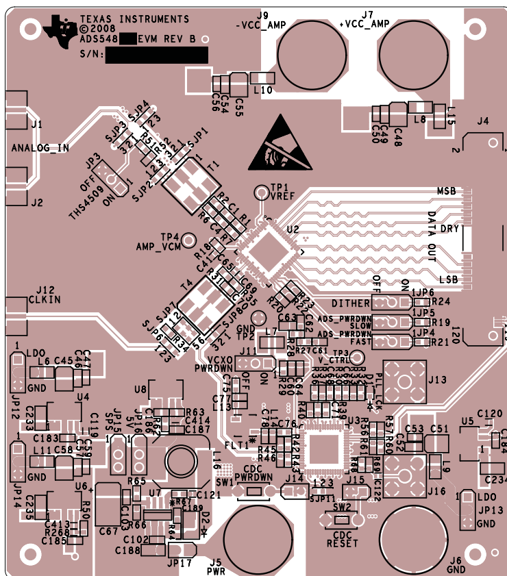
Figure 14. Component Side
