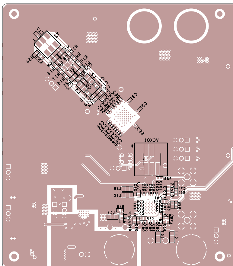
Figure 19. Bottom Side
