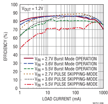
1A Buck Regulators, Efficiency vs Load
