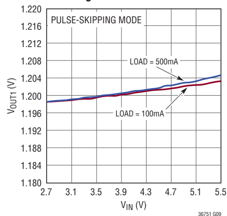
1A Buck Regulators, Line Regulation
