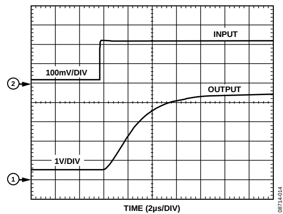
Figure 14. Rise Time
