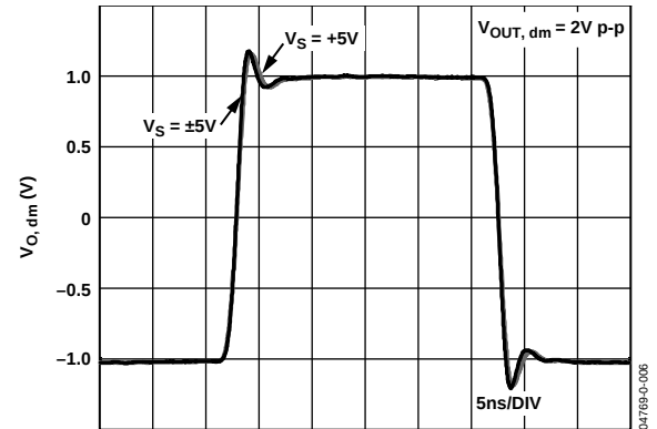
Figure 15. Large Signal Transient Response for Various Power Supply Voltages
