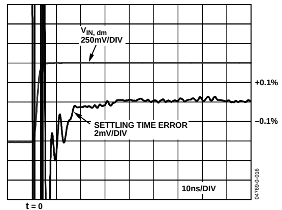
Figure 16. Settling Time (0.1%)
