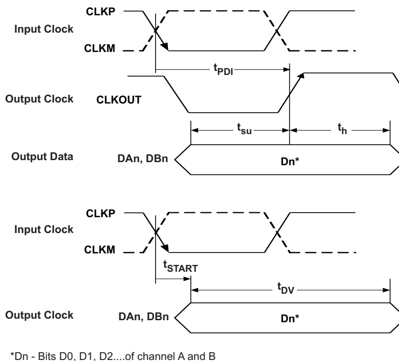
Figure 5. CMOS Interface Timing
