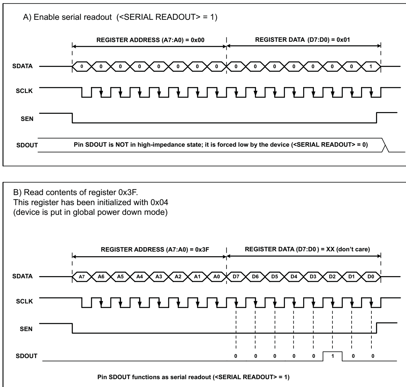
Figure 8. Serial Readout
