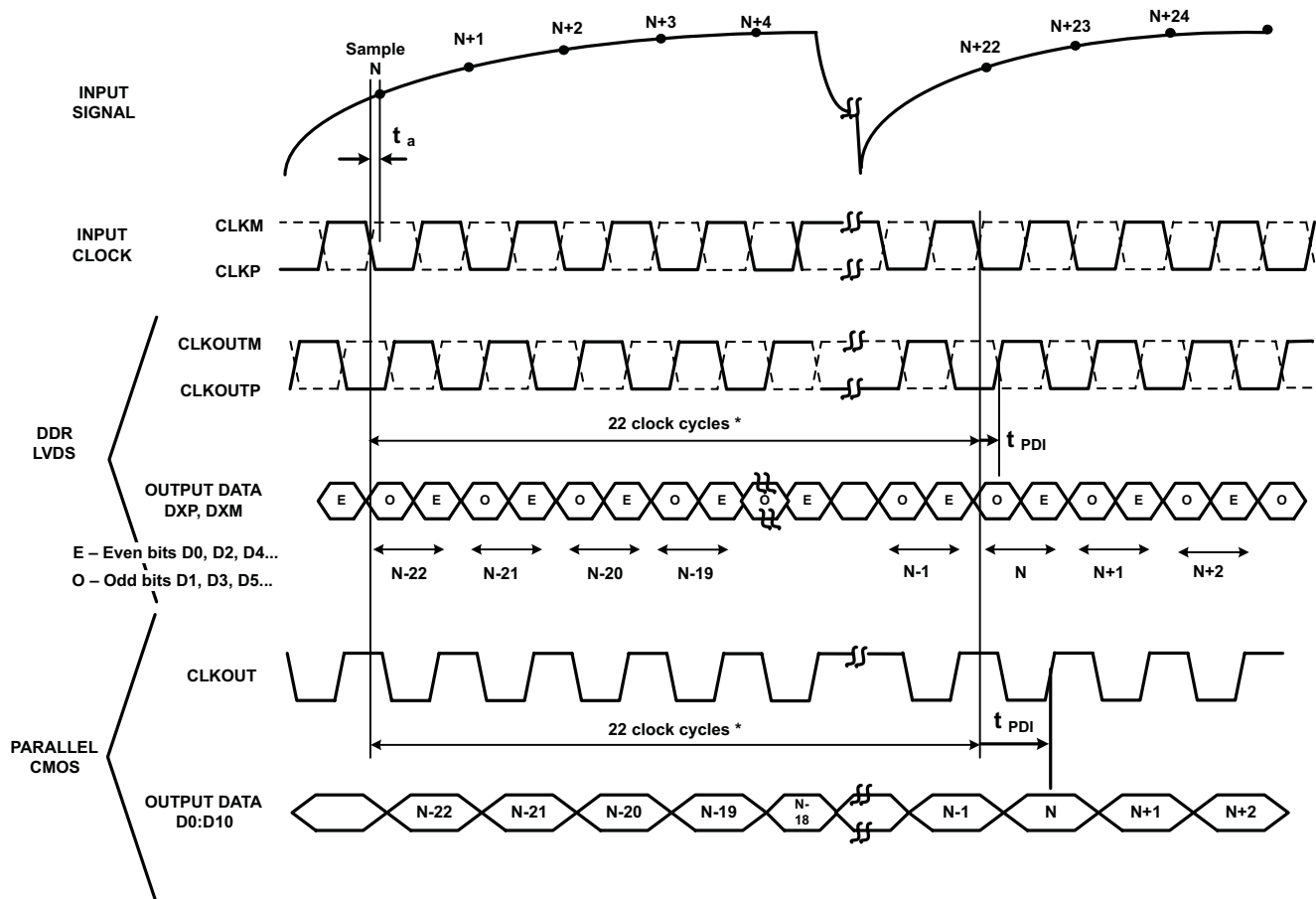
Figure 3. Latency Diagram
