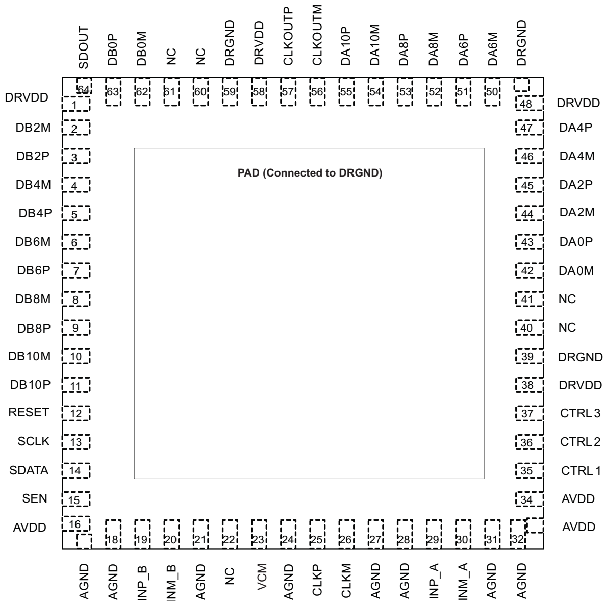
Figure 10. Pin Configuration
