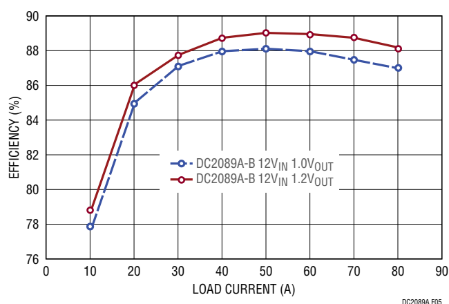
Figure 5. Typical Efficiency Curves DC2089A-B, F_{SW} = 350\text{kHz}
