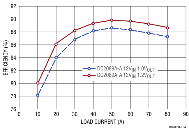
Figure 4. Typical Efficiency Curves DC2089A-A, F_{SW} = 350\text{kHz}
