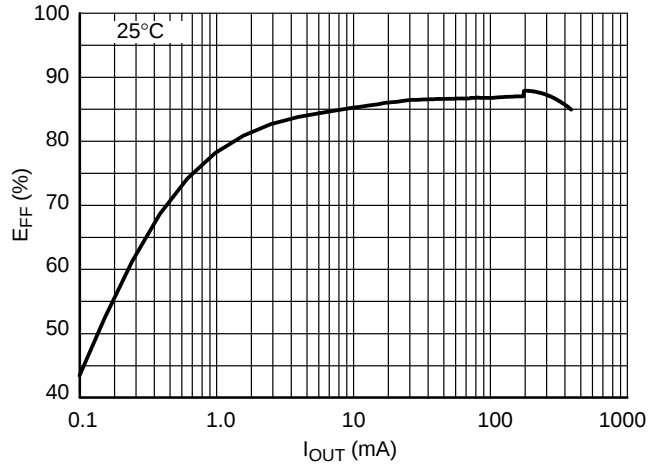
Figure 9. Efficiency versus IOUT (Auto Mode) L = 1 \mu\text{H} (TOKO DFE2016), V_{\text{IN}} = 3.6 \text{ V} , V_{\text{OUT}} = 1.2 \text{ V} , C_{\text{IN}} = 2.2 \mu\text{F} , C_{\text{OUT}} = 10 \mu\text{F}
