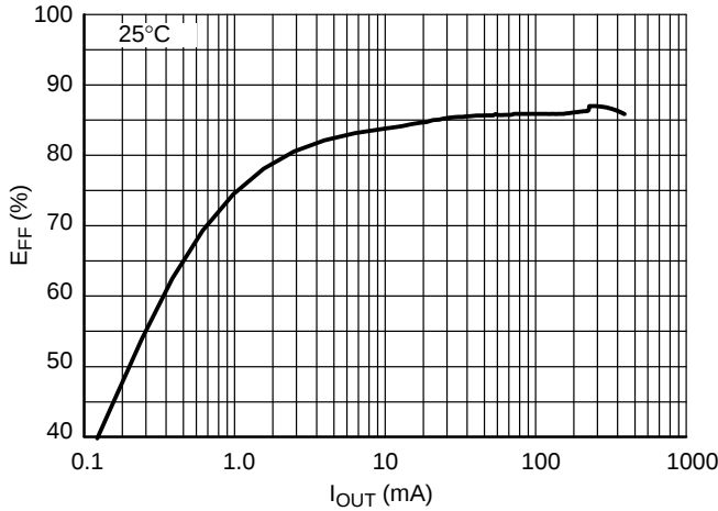
Figure 8. Efficiency versus IOUT (Auto Mode) L = 1 \mu\text{H} (TOKO DFE2016), V_{\text{IN}} = 5 \text{ V} , V_{\text{OUT}} = 1.2 \text{ V} , C_{\text{IN}} = 2.2 \mu\text{F} , C_{\text{OUT}} = 10 \mu\text{F}
