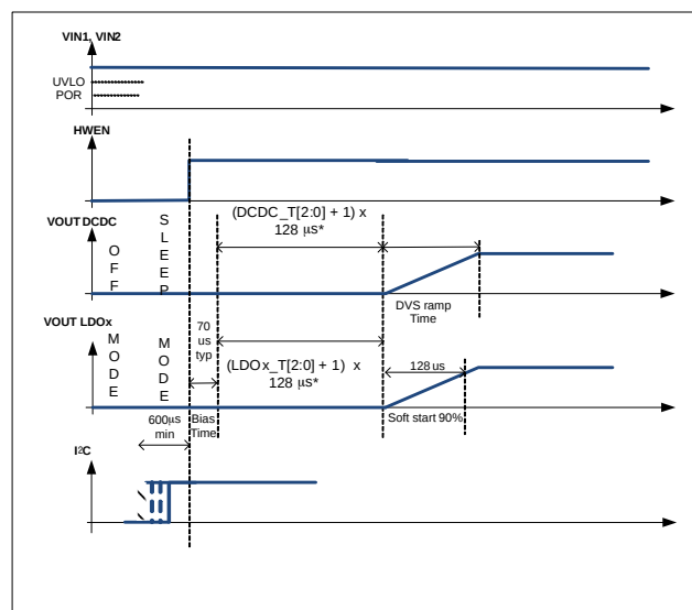
Figure 4. Sleep Mode PUS (SMPUS)
