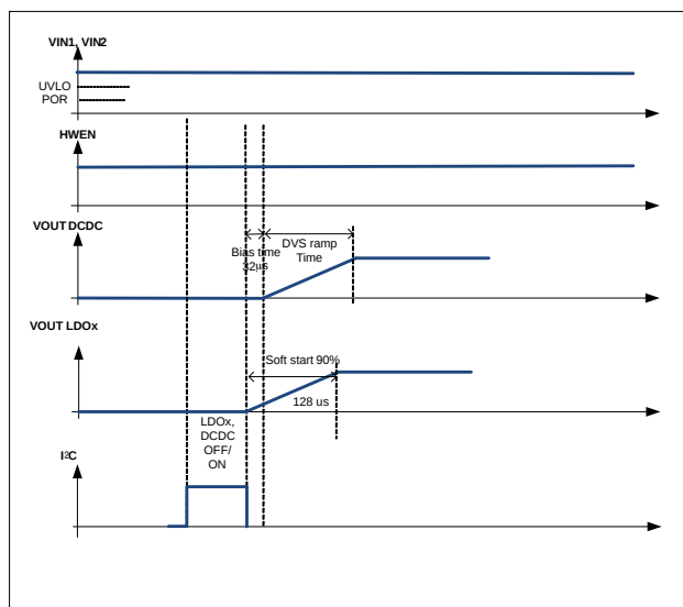
Figure 5. ON Mode PUS (OPUS)
