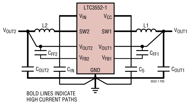
Figure 5. Layout Diagram
