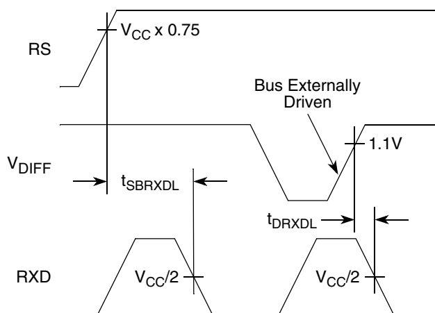
Figure 17. Timing Diagram for FlexCAN Standby Signal
