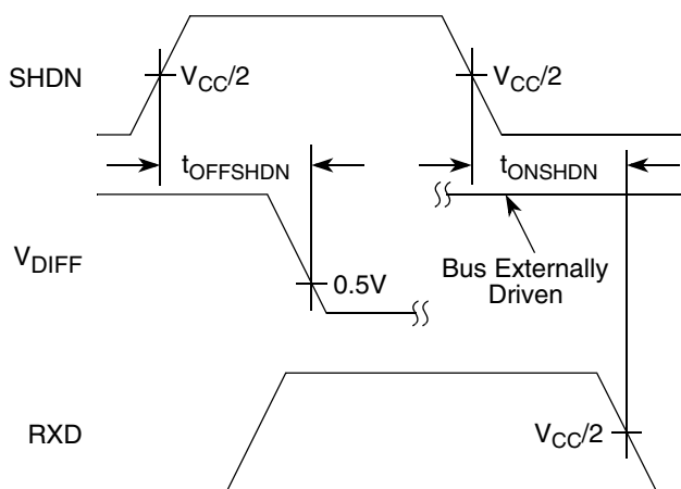
Figure 18. Timing Diagram for FlexCAN Shutdown Signal
