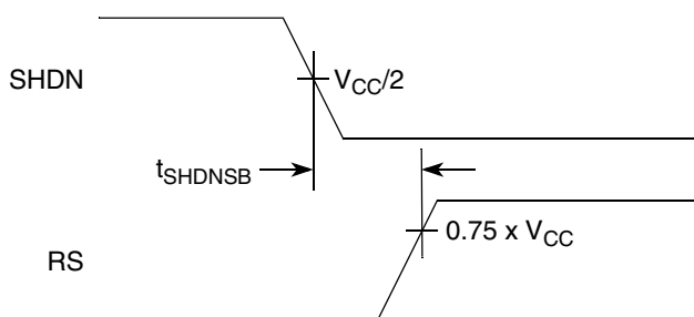
Figure 19. Timing Diagram for FlexCAN Shutdown-to-Standby Signal
