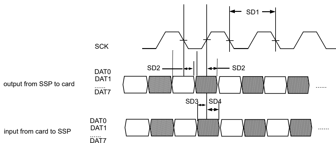
Figure 37. MMC4.4 Timing
