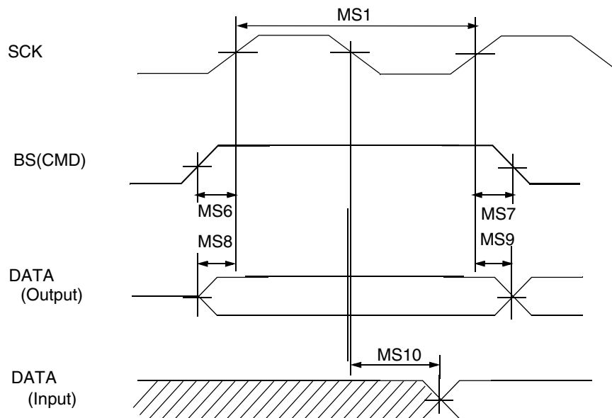
Figure 39. MS Serial Transfer Mode Timing Diagram
