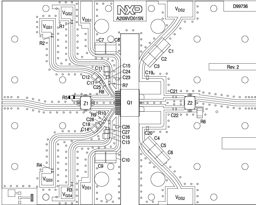
Figure 4. A2I09VD015NR1 Characterization Test Circuit Component Layout — 920–960 MHz
