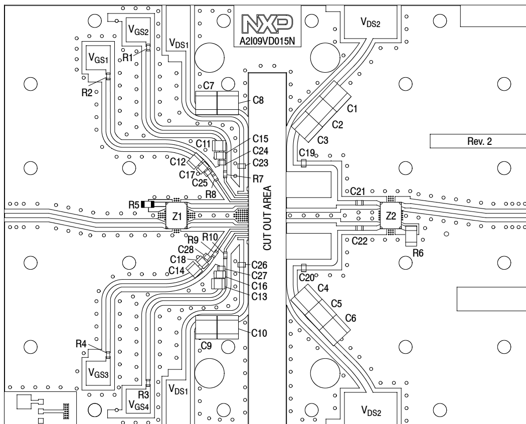
Figure 3. A2I09VD015NR1 Production Test Circuit Component Layout
