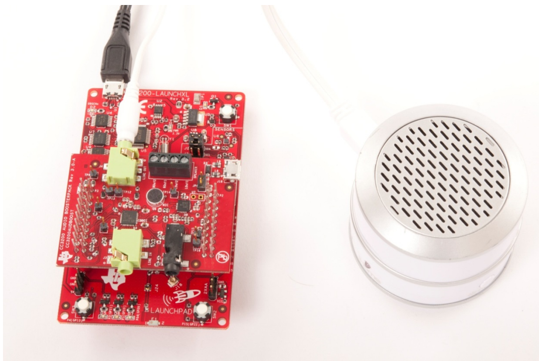
Figure 2-4. Connected Boards
