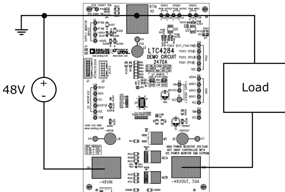
Figure 1. LTC4284 Setup
