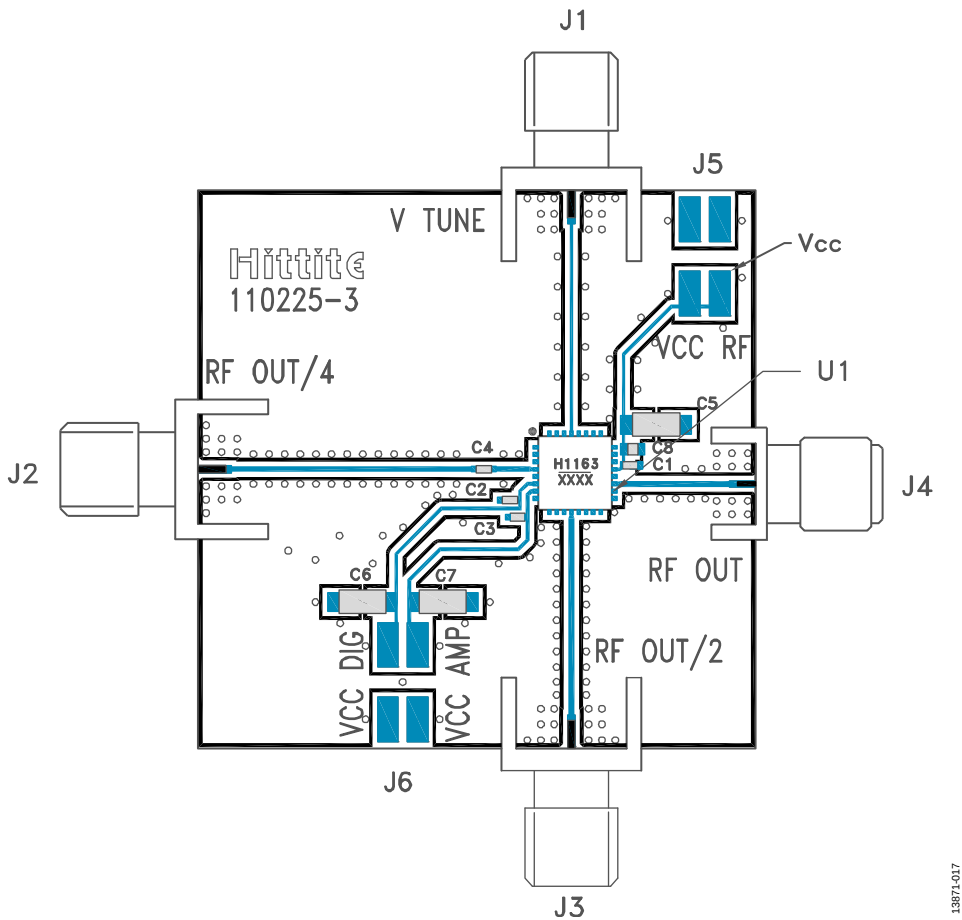
Figure 17. Evaluation PCB
