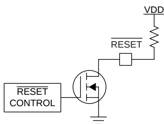
Figure 35. Open-Drain \overline{\text{RESET}} Configuration
