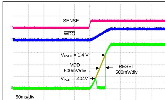
Figure 36. Startup Waveform
