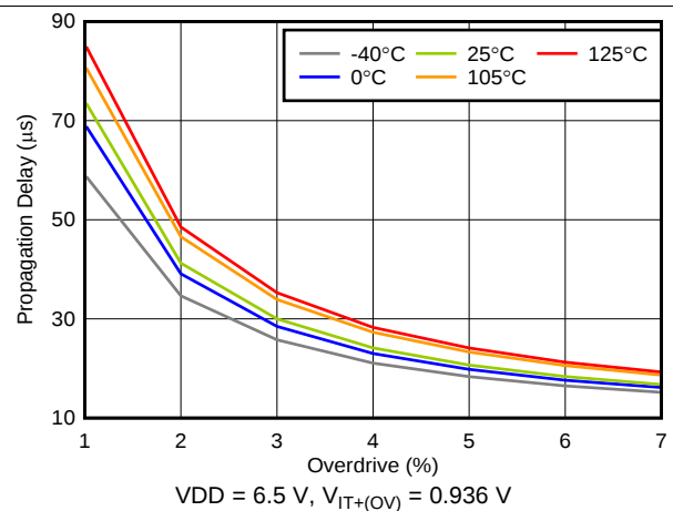
Figure 15. Propagation Delay vs Overdrive
