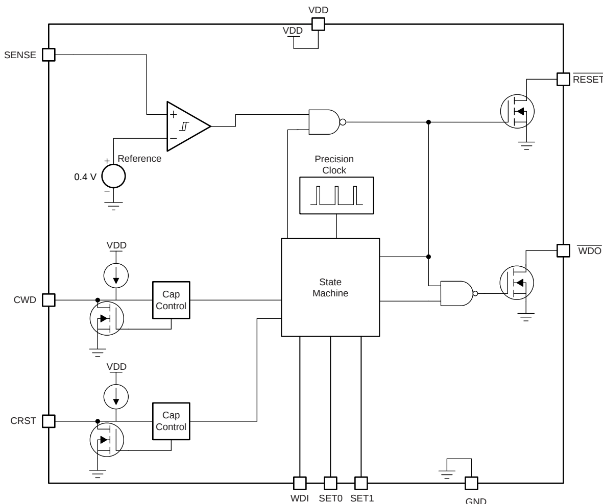
Figure 23. Adjustable Version Block Diagram
