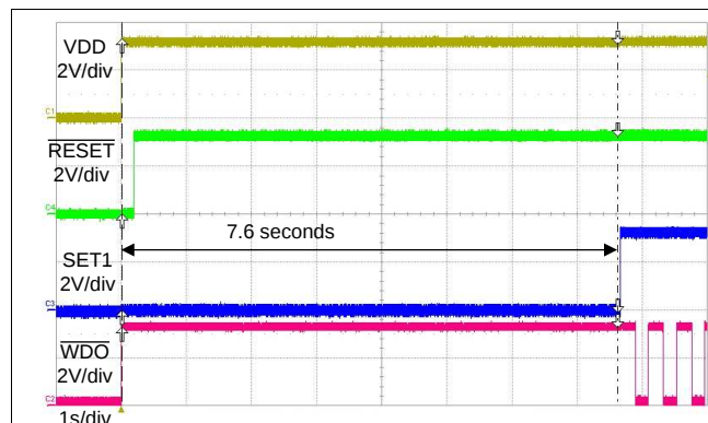
Figure 42. Startup Without a WDI Signal
