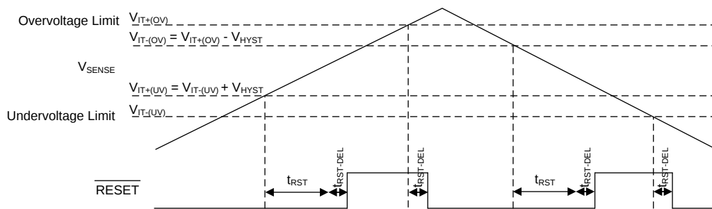
Figure 24. Window Comparator Timing Diagram
