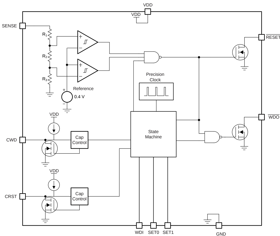
Figure 22. Fixed Version Block Diagram
