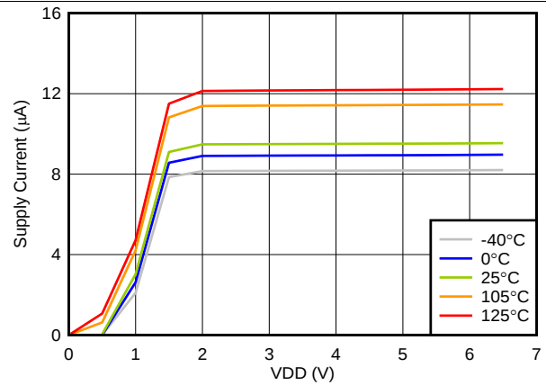
Figure 11. Supply Current vs Power-Supply Voltage
