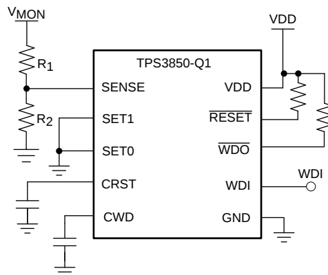
Figure 25. Adjustable Voltage Monitor
