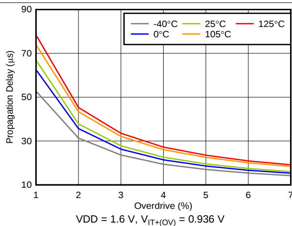
Figure 14. Propagation Delay vs Overdrive
