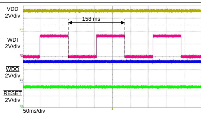
Figure 43. Typical WDI Signal
