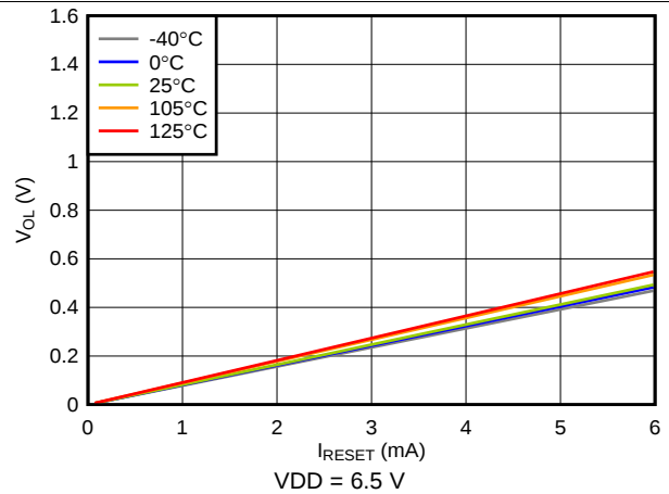
Figure 13. Low-Level \overline{\text{RESET}} Voltage vs \overline{\text{RESET}} Current
