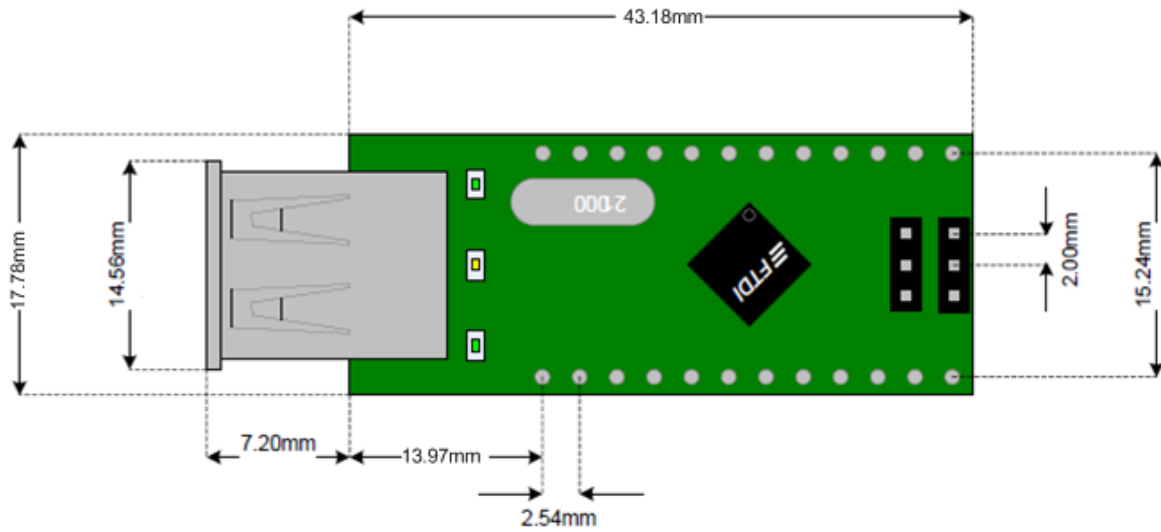
Figure 5.1 VDIP1 Dimensions (Top View)
