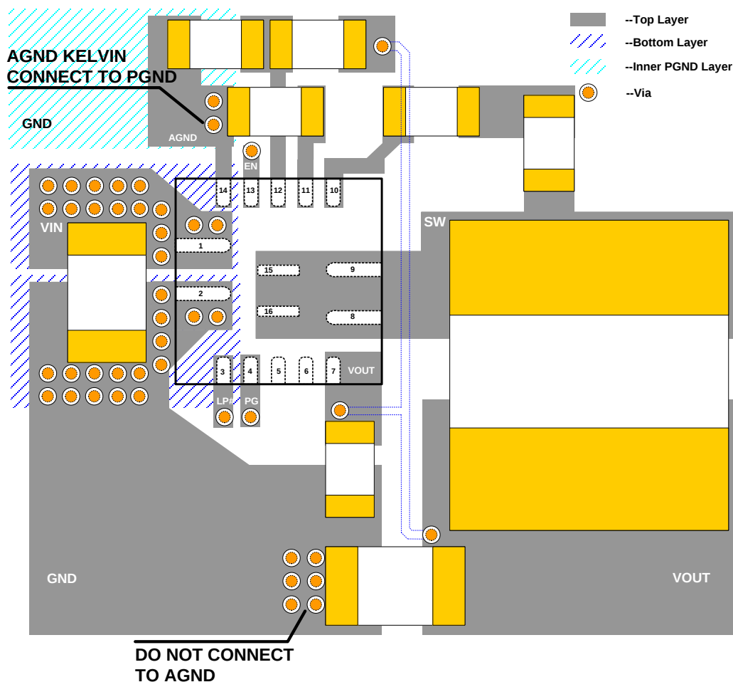
Figure 13—Recommend Layout
