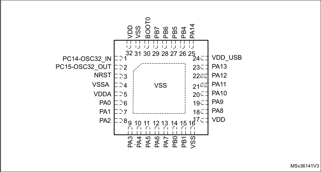
Figure 6. STM32L082xx UFQFPN32 pinout
