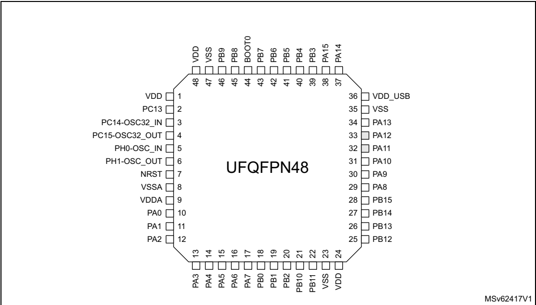
Figure 4. STM32L082xx UFQFPN48
