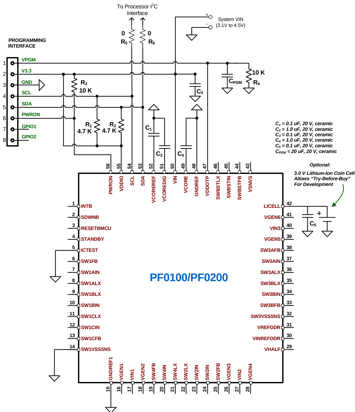
Figure 4. PF Device Minimum System for Programming
