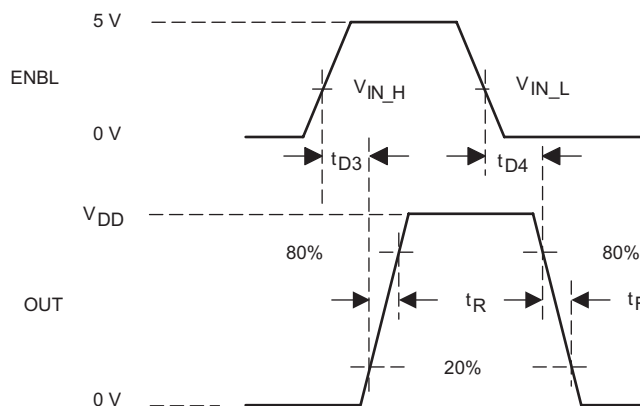
Figure 9. Switching Waveforms for Inverting Driver (a) and Non-Inverting Driver (b)
