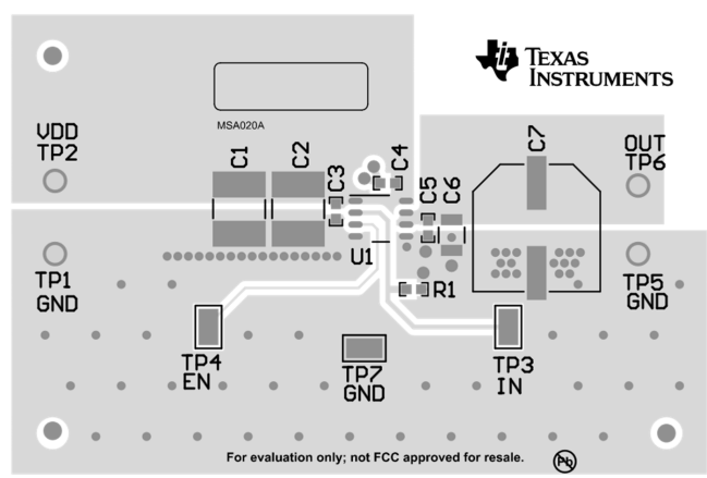
Figure 5. Layout - Top Composite
