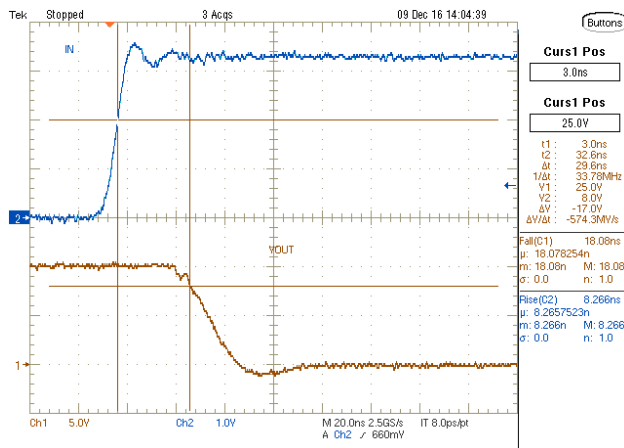
Figure 11. UCC27321-Q1 IN vs Output PWM Propagation Delay (High)
