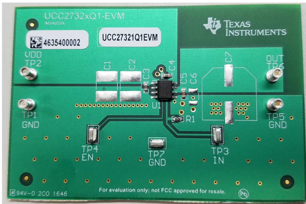
Figure 1. UCC2732xQ1EVM Board (Photo)
