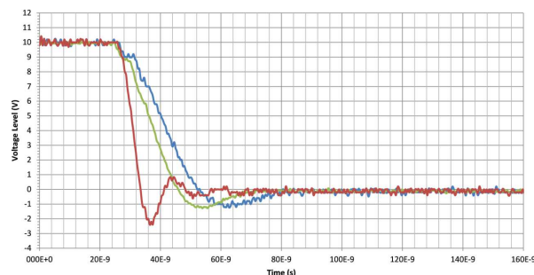
Figure 15. UCC27321-Q1 OUT vs Load Capacitance ( V_{IN} = 10\text{ V} )
