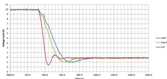
Figure 18. UCC27322-Q1 OUT vs Load Capacitance
