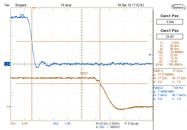
Figure 14. UCC27321-Q1 EN vs Output PWM Propagation Delay (Low)
