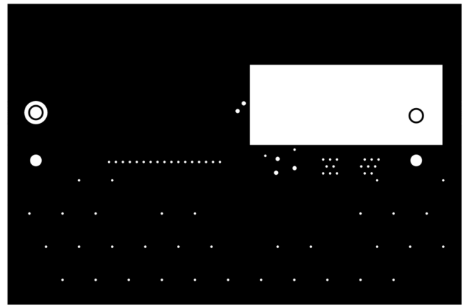
Figure 8. Bottom Layer
