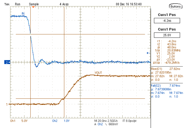
Figure 12. UCC27321-Q1 IN vs Output PWM Propagation Delay (Low)
