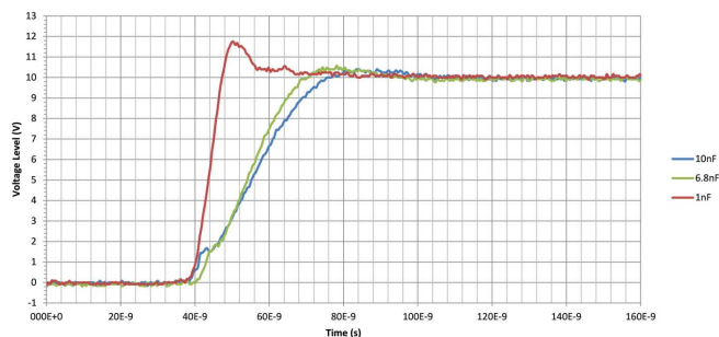
Figure 16. UCC27321-Q1 OUT vs Load Capacitance
