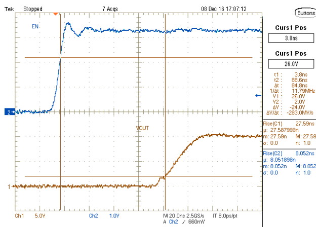
Figure 13. UCC27321-Q1 EN vs Output PWM Propagation Delay (High)
