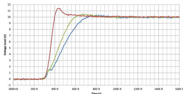
Figure 17. UCC27322-Q1 OUT vs Load Capacitance ( V_{IN} = 10\text{ V} )
