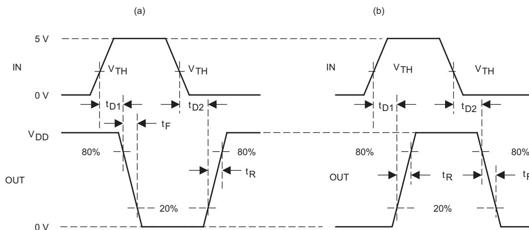
Figure 9. Switching Waveforms for Inverting Driver (a) and Non-Inverting Driver (b)
