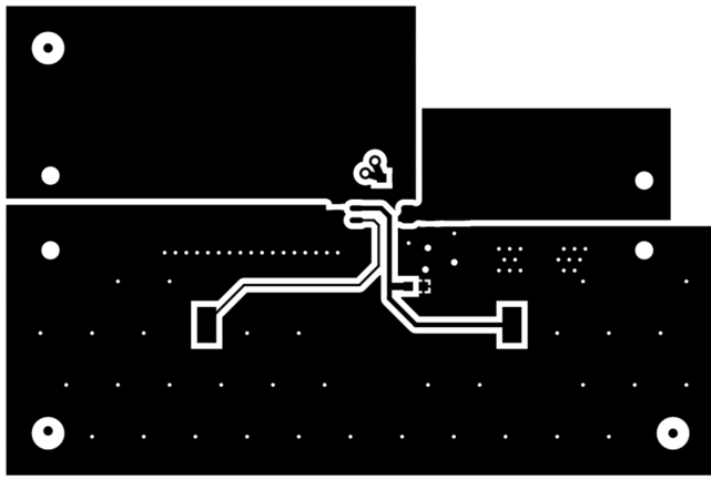
Figure 7. Top Layer
