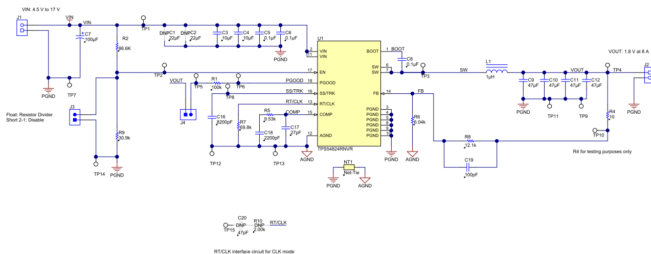
Figure 24. TPS54824EVM-779 Schematic
