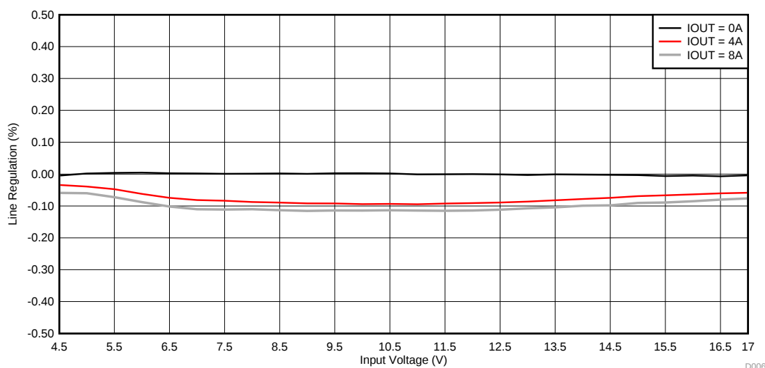
Figure 5. TPS54824EVM-779 Line Regulation
