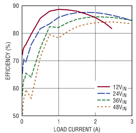
Efficiency, V_{OUT} = -8\text{V} , BIAS Tied to LTM8073 GND
