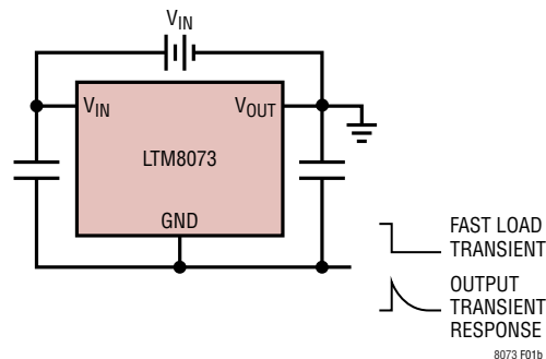
Figure 1b. Any Output Voltage Transient Appears on LTM8073 GND
