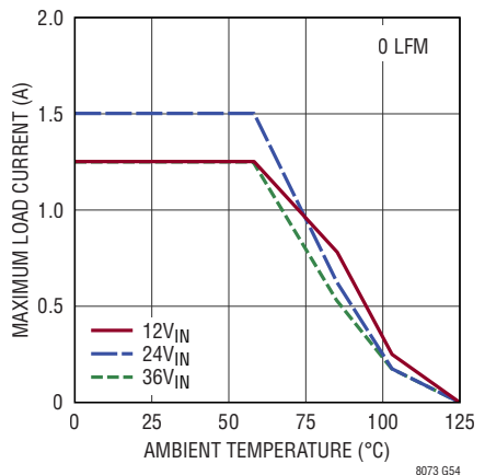
Derating, I-Grade V_{OUT} = -15\text{V} , BIAS Tied to LTM8073 GND, DC2389A Demo Board
