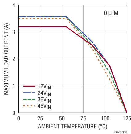
Derating, V_{OUT} = -3.3\text{V} , BIAS Tied to LTM8073 GND, DC2389A Demo Board
