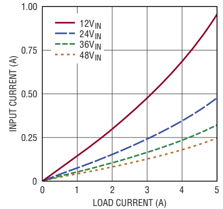
Input vs Load Current V_{OUT} = 1.5\text{V}
