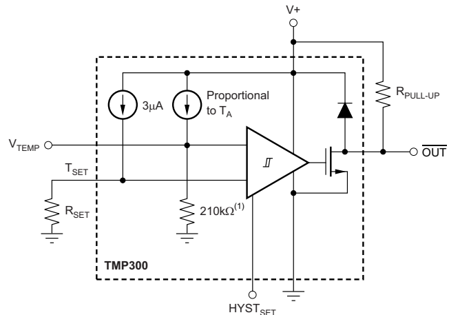
Application Schematic
