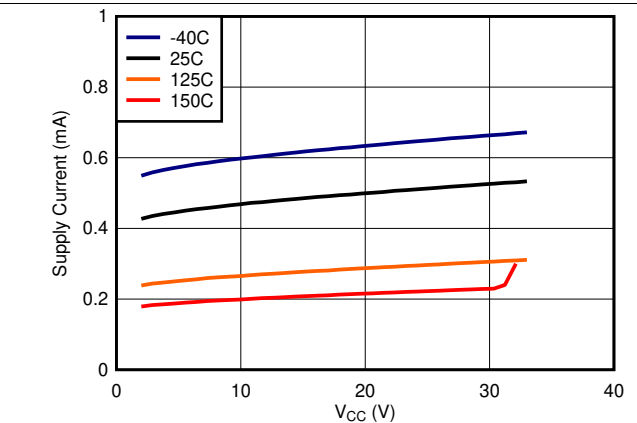
Figure 2. Supply Current vs. Supply Voltage LM2903E-Q1 Only
