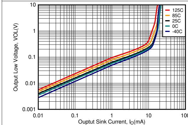
Figure 5. Output Low Voltage vs. Output Current
