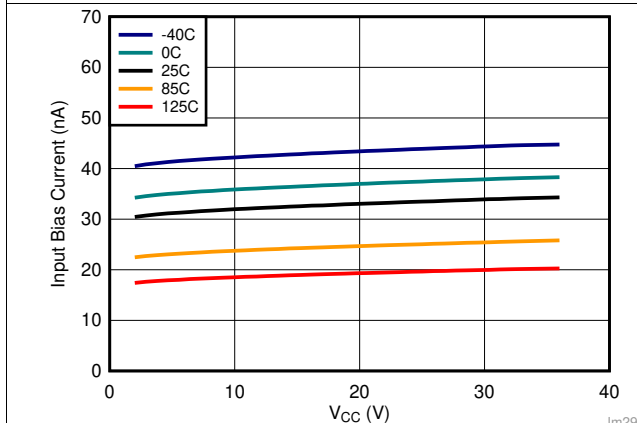
Figure 3. Input Bias Current vs. Supply Voltage
