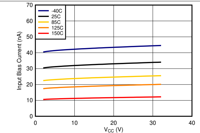
Figure 4. Input Bias Current vs. Supply Voltage LM2903E-Q1 Only
