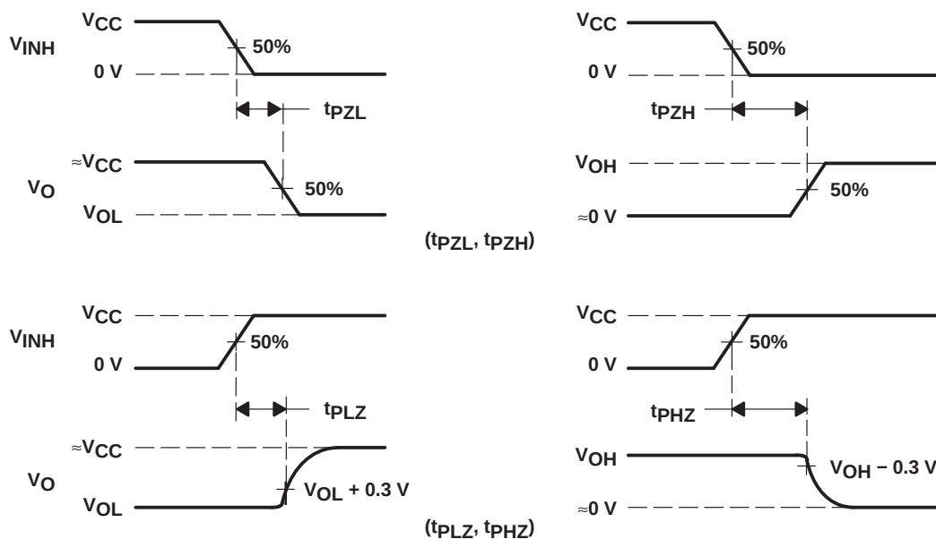
VOLTAGE WAVEFORMS
