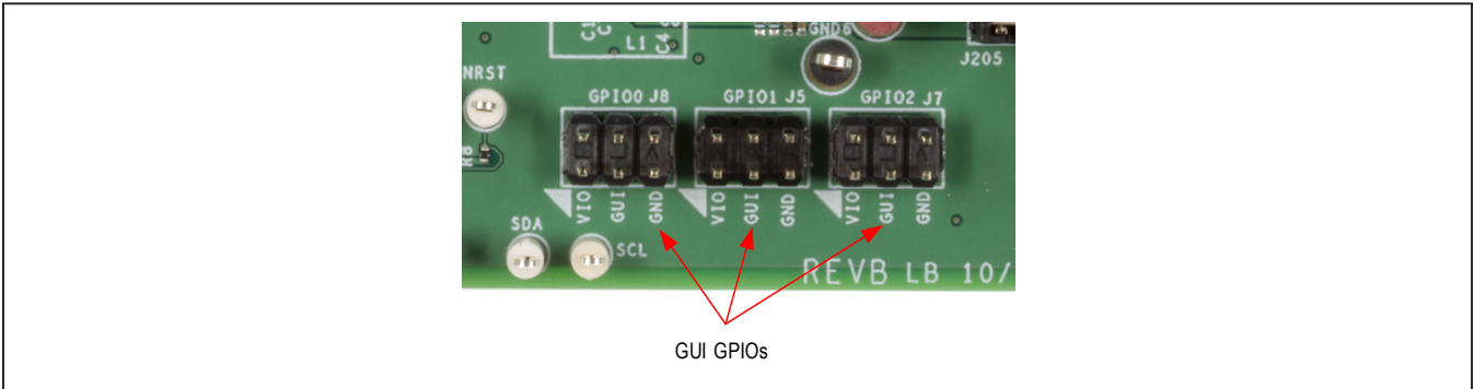
Figure 7. GPIO Headers
