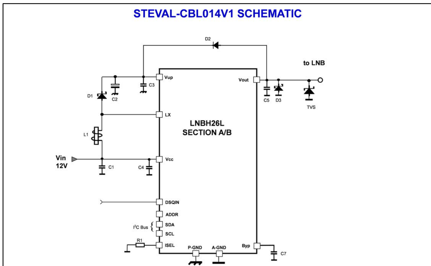
Figure 1: STEVAL-CBL014V1 schematic
