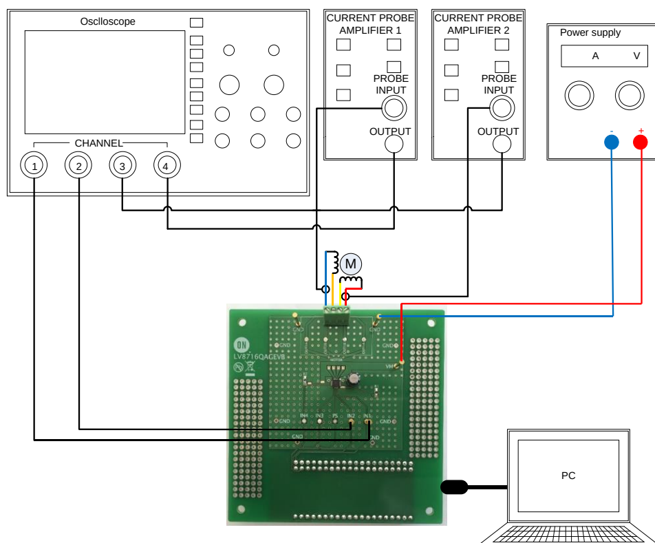
Figure 31. Setup for a stepper motor
