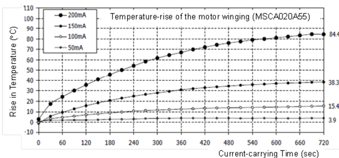
Figure 6. Temperature-rise characteristic of the motor winding
