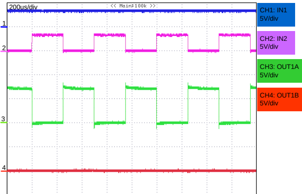
Figure 40. Forward<->Brake
