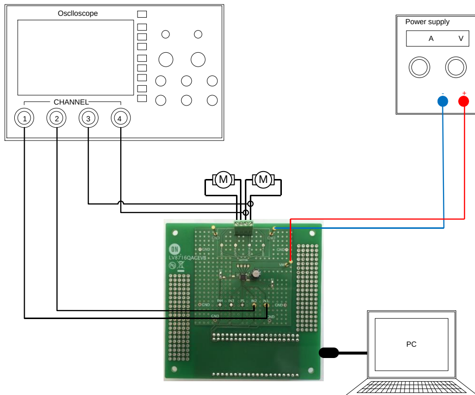
Figure 36. Setup for a brush DC motor
