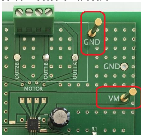
Figure 2. DC power supply
