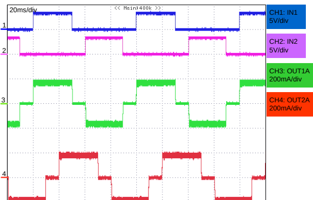
Figure 35. Half step setting waveform
