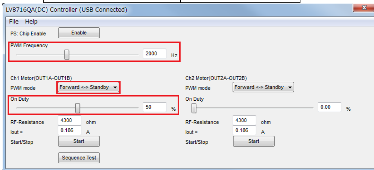
Figure 38. Setting parameter of GUI for brush DC motor
