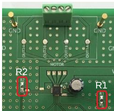
Figure 5. RF resistor
