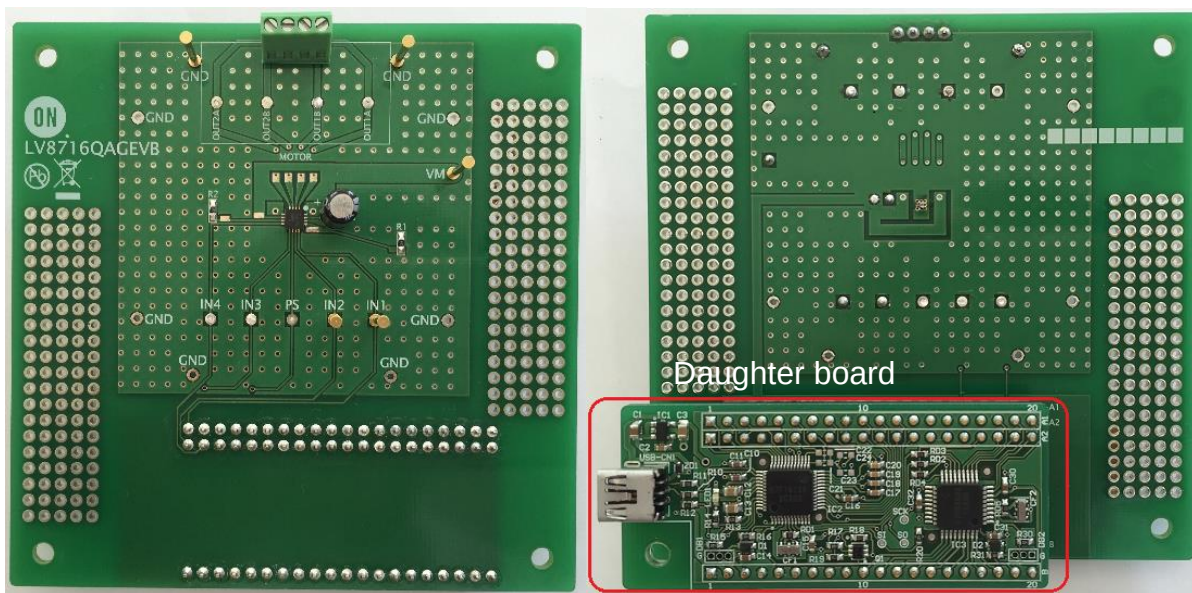
LV8716QAGEVB top view
