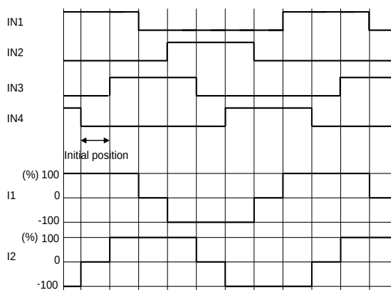
Figure 22. Half step (CW)
