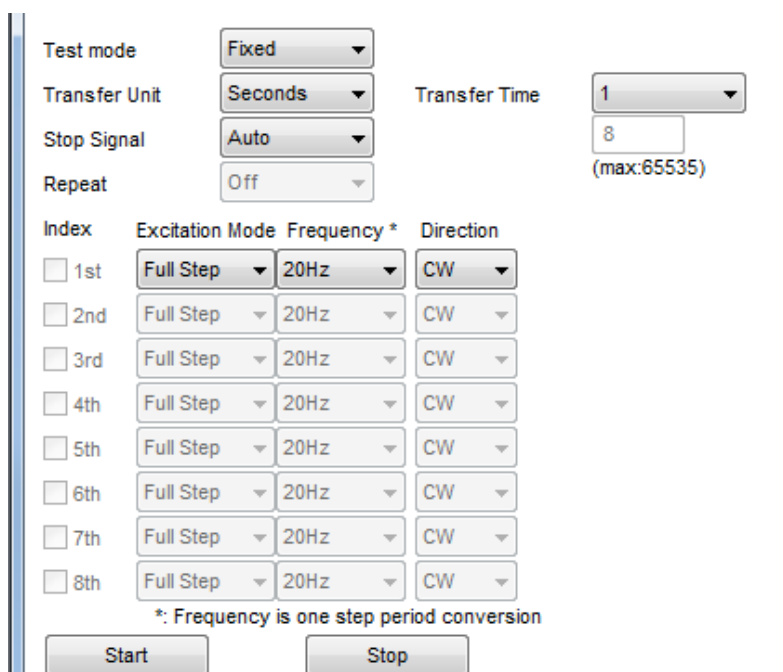
Figure 19. GUI field description of stepper controller window 1-2
