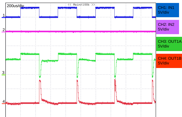
Figure 39. Forward<->Standby
