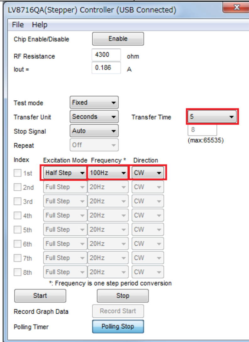
Figure 33. Setting parameter of GUI for Stepper mode
