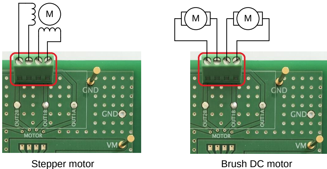
Figure 3. Motor winding connector
