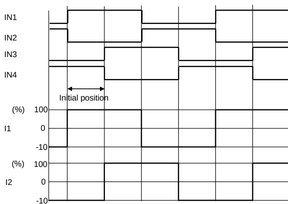
Figure 21. Full step (CW)
