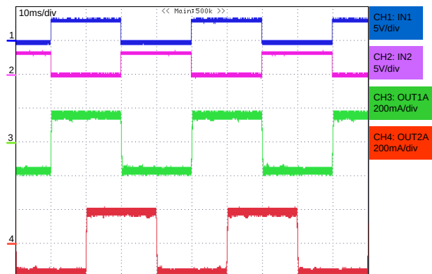
Figure 34. Full step setting waveform
