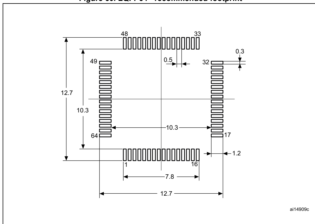
Figure 60. LQFP64 - recommended footprint
