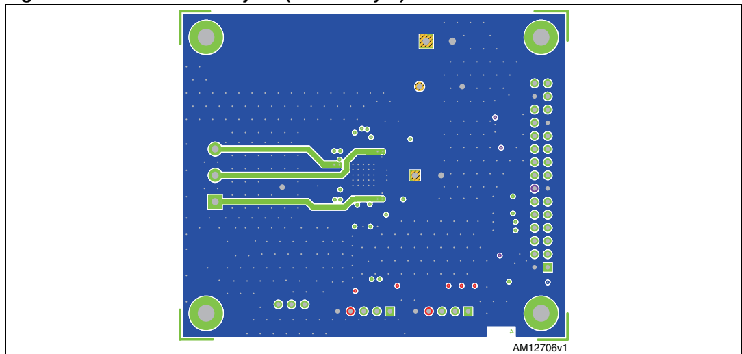
Figure 7. EVAL6235Q - layout (bottom layer)
