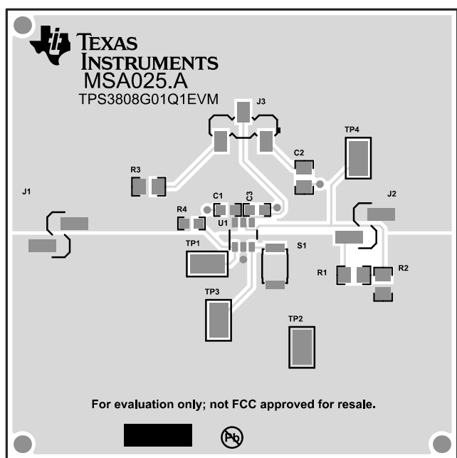
Figure 5. Layout—Top
