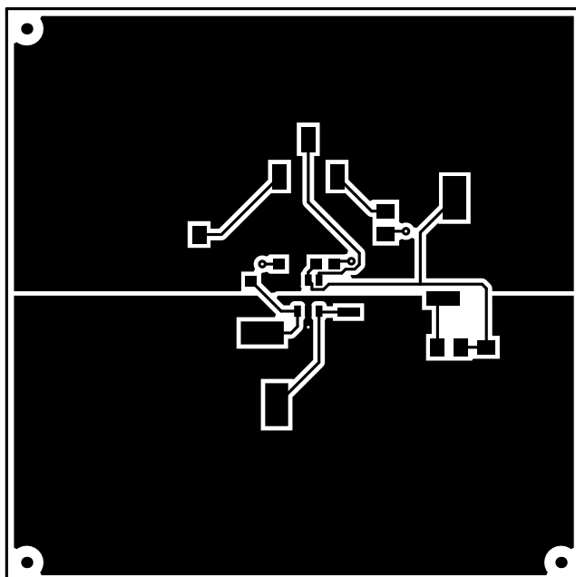
Figure 7. Top Layer
