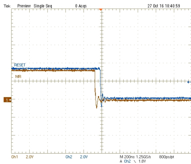
Figure 11. TPS3808G01-Q1 \overline{RESET} Asserted Due to \overline{MR} Pulled Low
