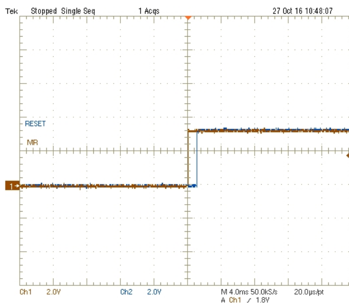
Figure 13. TPS3808G01-Q1 \overline{RESET} Deasserted Due to \overline{MR} Pulled High, With Delay t_D , C_T Tied to GND Through 100-pF capacitor
