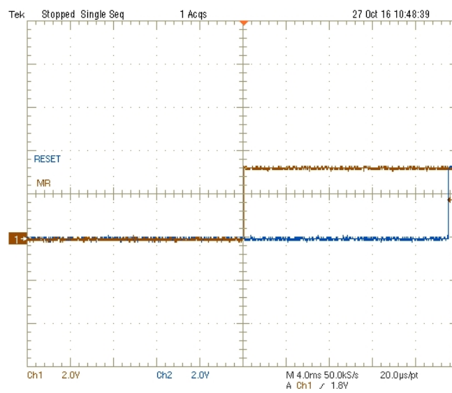
Figure 12. TPS3808G01-Q1 \overline{RESET} Deasserted Due to \overline{MR} Pulled High, With Delay t_D , C_T Floating
