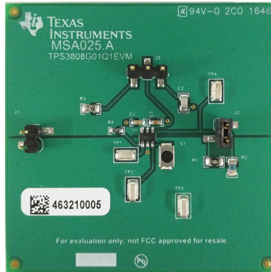
Figure 1. TPS3808G01-Q1EVM Board
