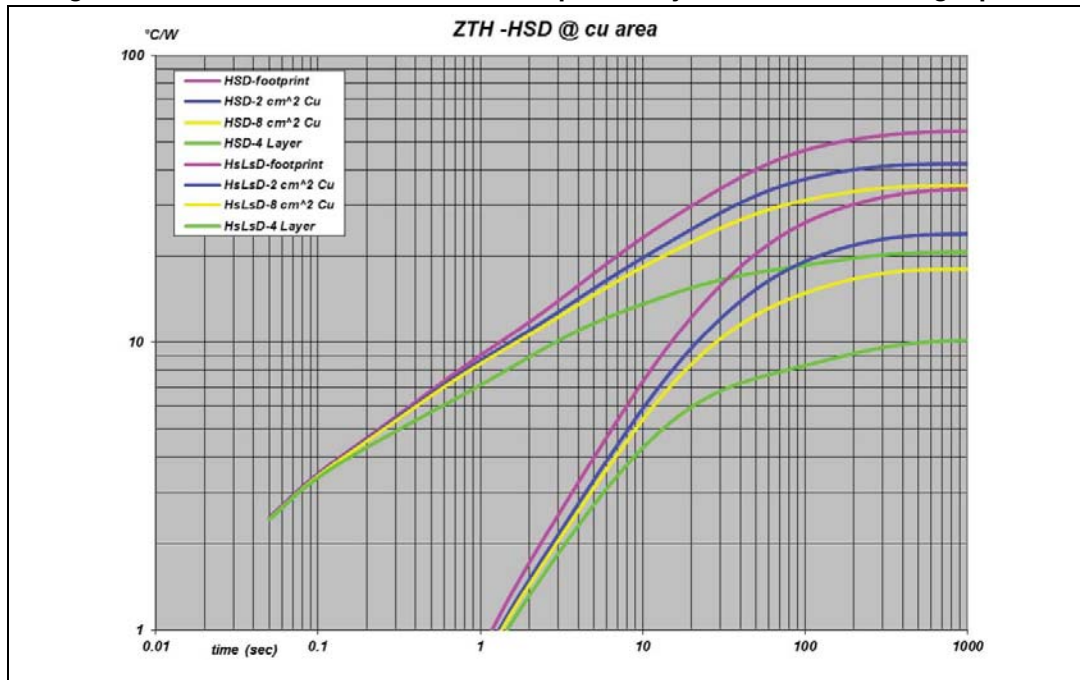
Figure 10. PowerSSO-36 HSD thermal impedance junction ambient single pulse
