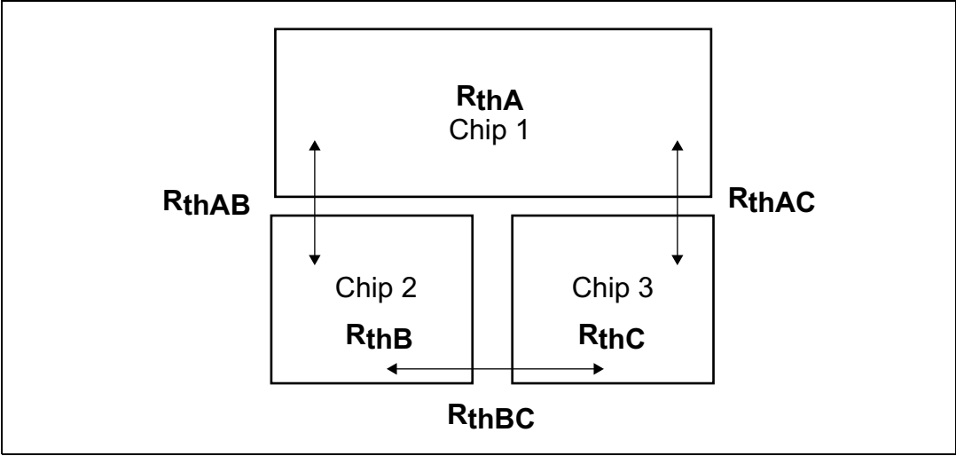
Figure 8. Chipset configuration
