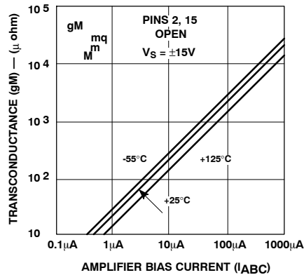
Figure 10. Transconductance
