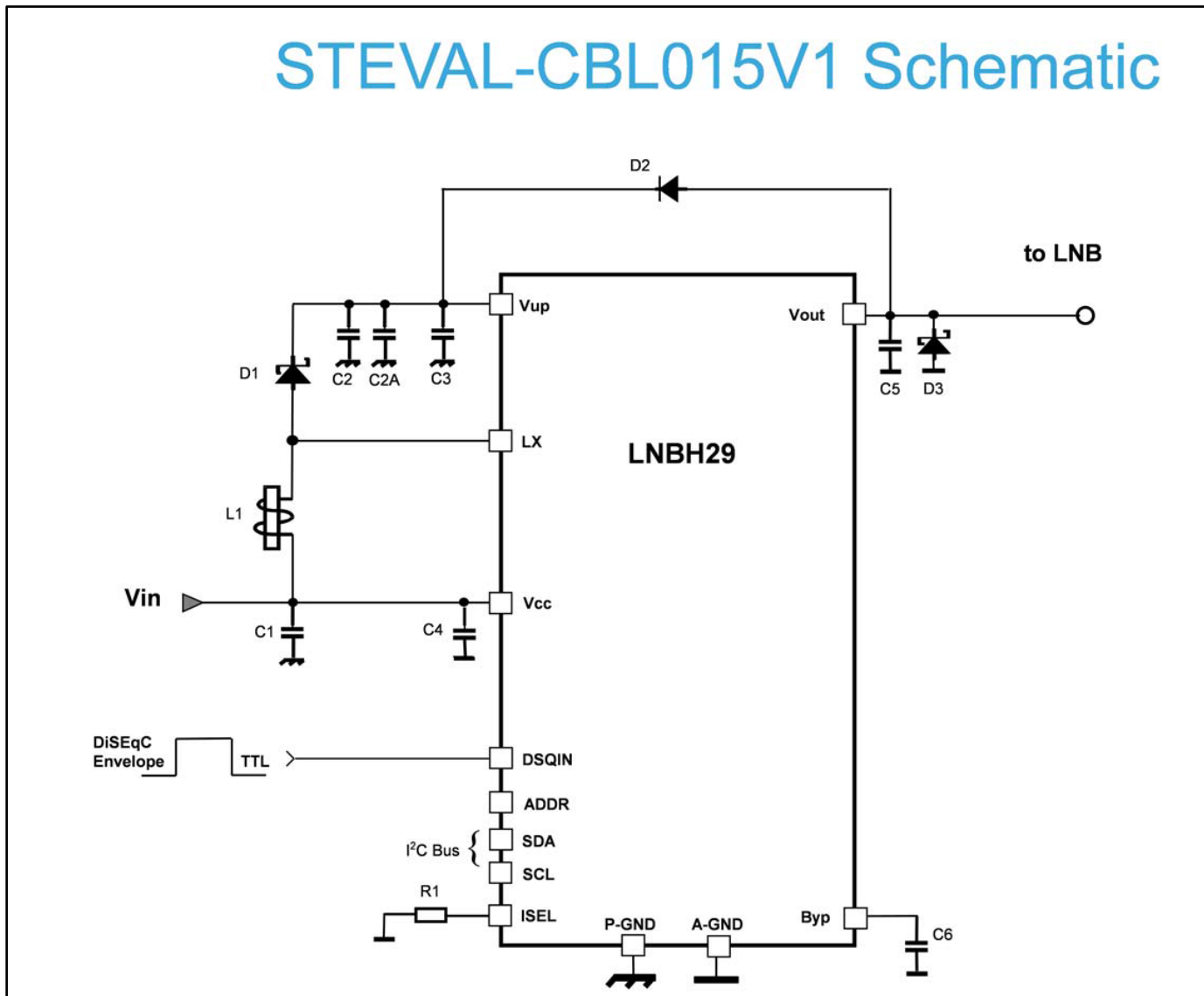
Figure 1: STEVAL-CBL015V1 schematic
