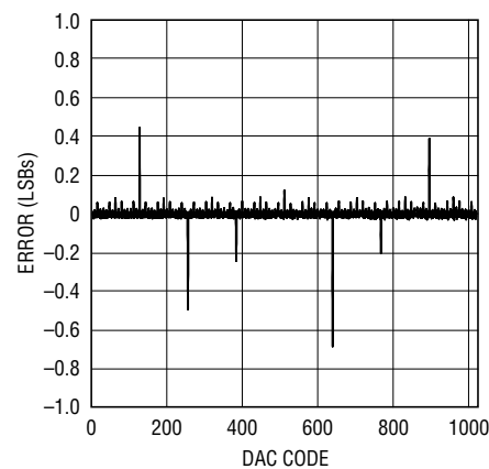
DAC-DNL
