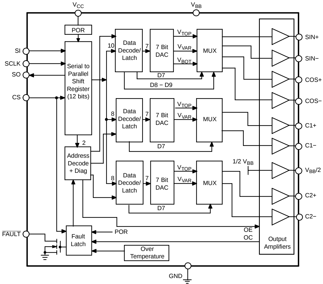
Figure 1. Block Diagram
