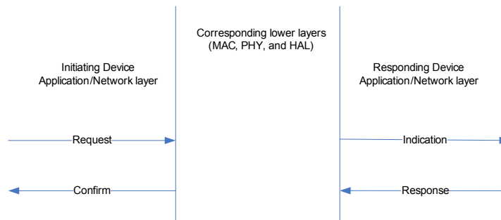
Figure 3-2. Layer Services
