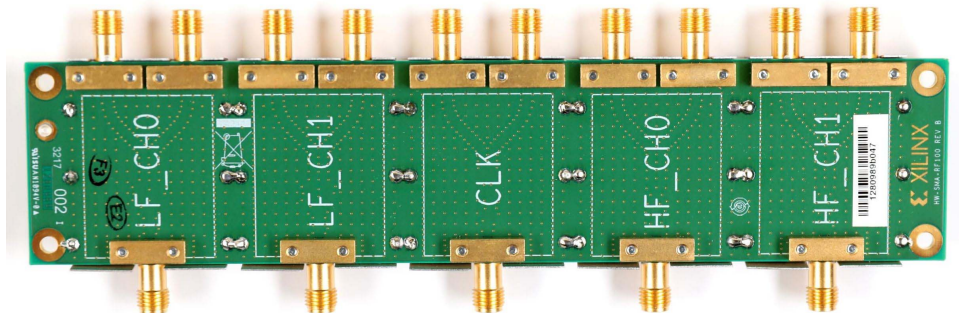
Figure 1-17: Balun Board—Bottom Side
