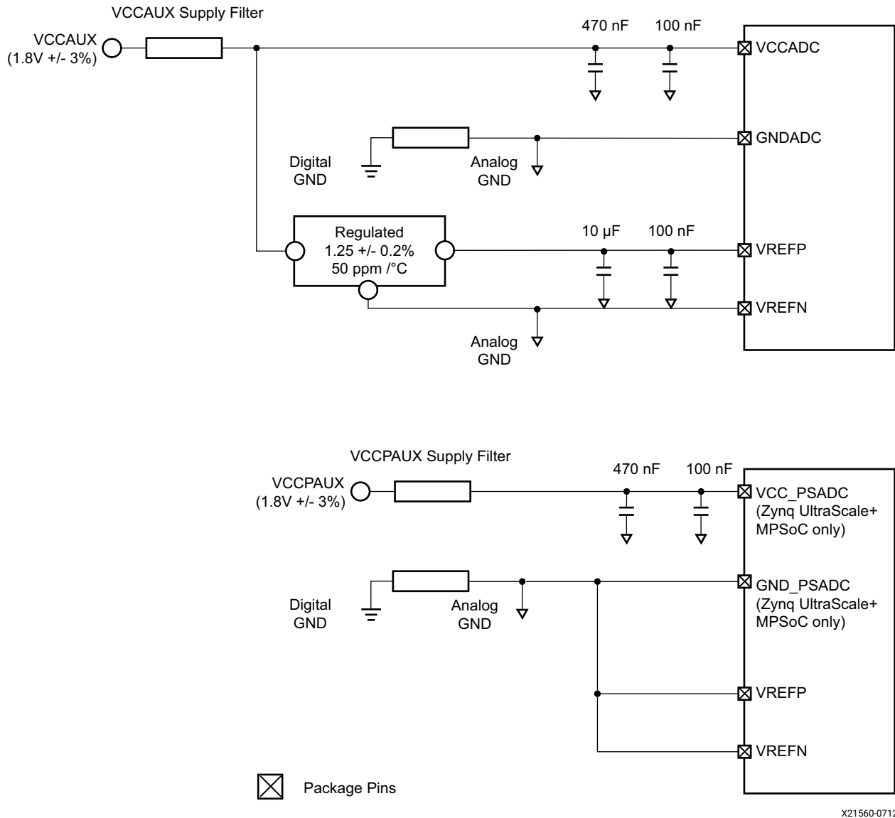
Figure 1-10: PL and PS SYSMON Power Connections
