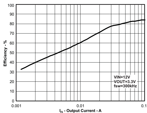
Figure 59. Light-Load Efficiency
