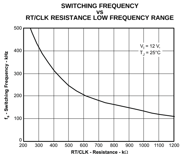
Figure 40. Low-Range RT
