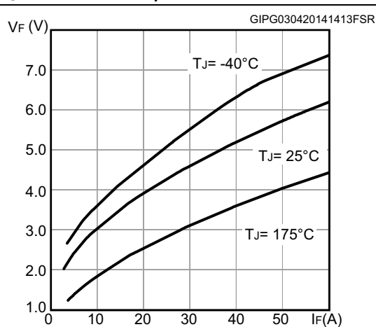
Figure 21. Diode V_F vs. forward current
