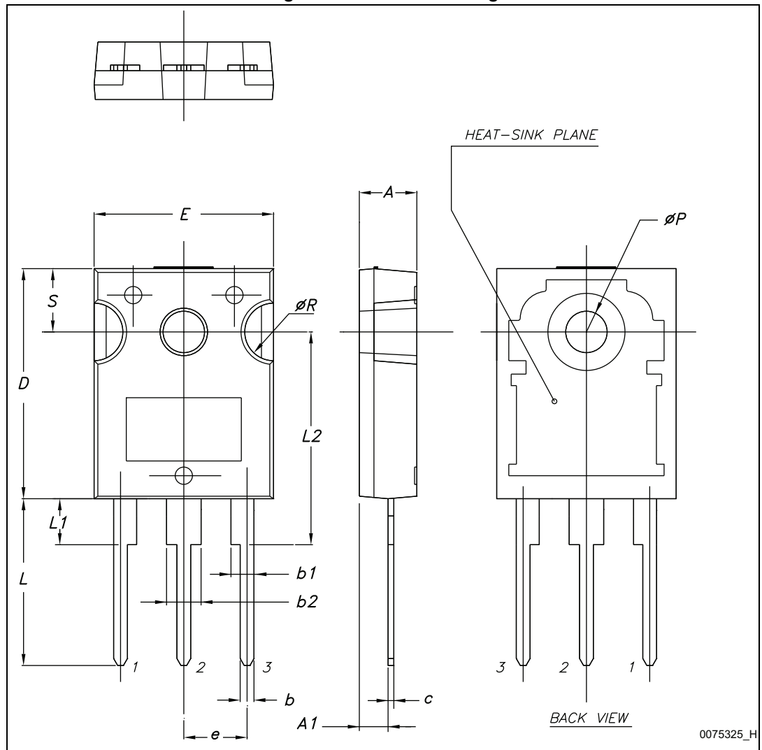
Figure 32. TO-247 drawing
