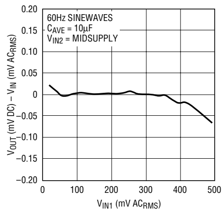
AC Linearity
