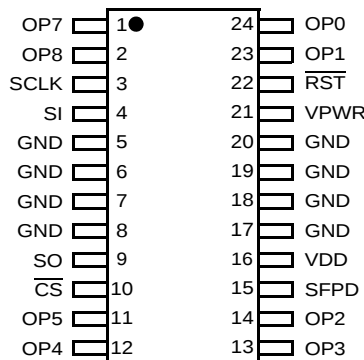
Figure 3. 33298 Pin Connections
