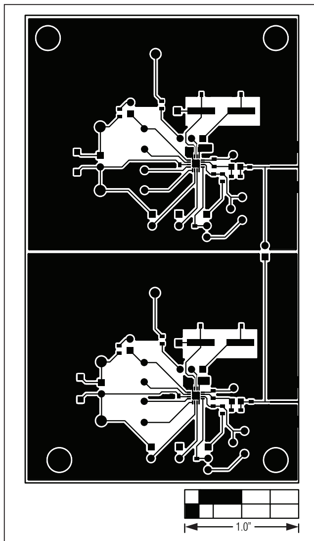
Figure 3. MAX9947 EV Kit PCB Layout—Component Side
