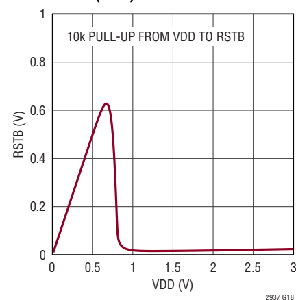
RSTB (Low) vs VDD
