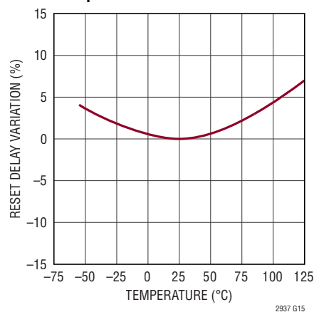
Reset Delay Variation vs Temperature
