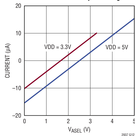
ASEL \overline{n} Current vs Input Voltage
