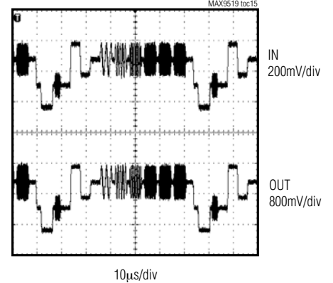
PAL MULTIBURST RESPONSE
